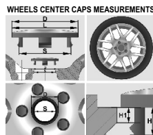
D - Outside diameter - Ø(mm) S - Rim hole diameter - Ø(mm) L - Sticker diameter - Ø(mm) H - Fixing length - (mm) H1 - Length up to fixing - (mm)
